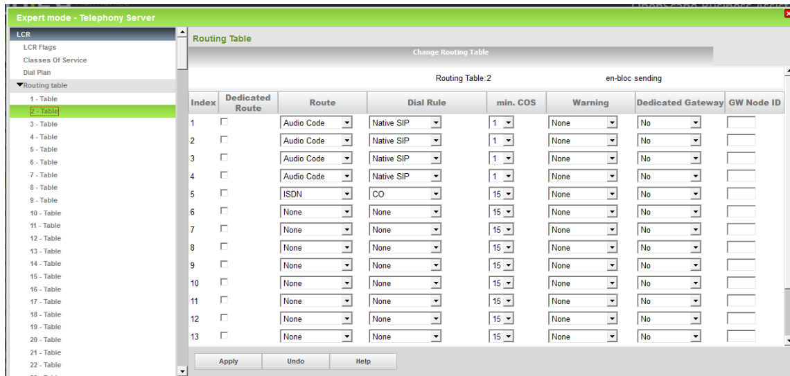
Figure 3-10: Routing Table
