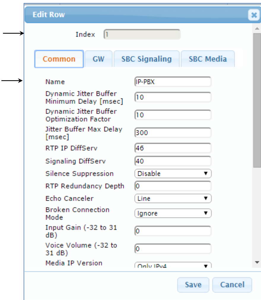
Figure 4-14: Configuring IP Profile for IP-PBX – Common Tab
