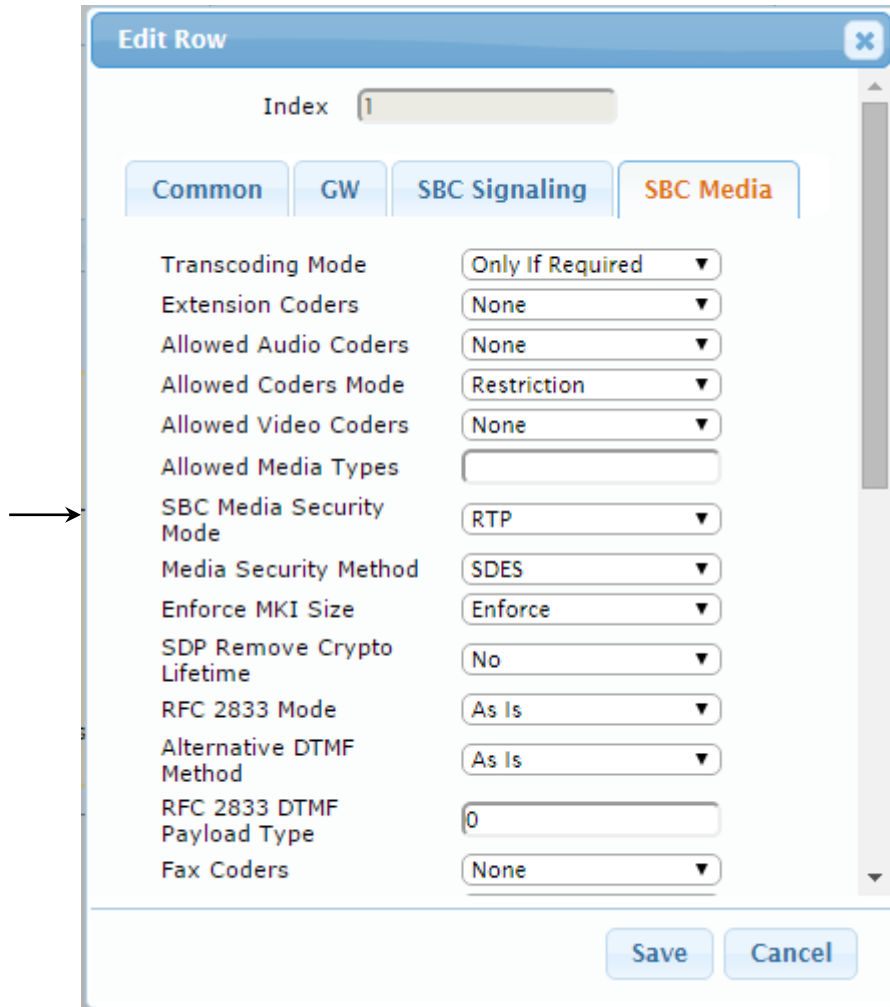
Figure 4-16: Configuring IP Profile for IP-PBX – SBC Media Tab
